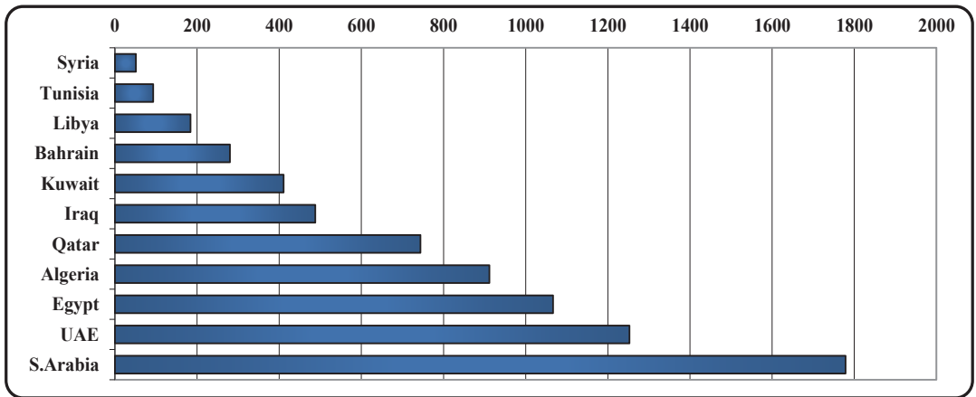
Natural gas consumption in OAPEC Members, 2019-2023 (Thousand boe/day)
