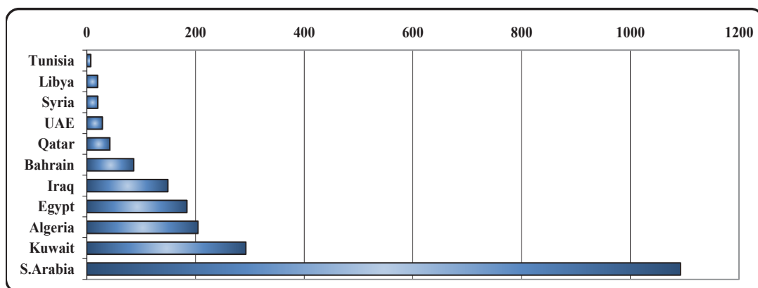
Production of gas oil and diesel in OAPEC Members, 2019-2023 (Thousand b/day)
