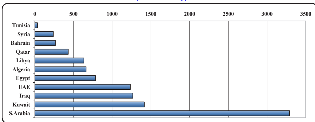
Installed refining capacities in OAPEC Members, 2019-2023 (Thousand b/day)
